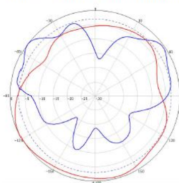
3300~6000MHz Typical pattern:
