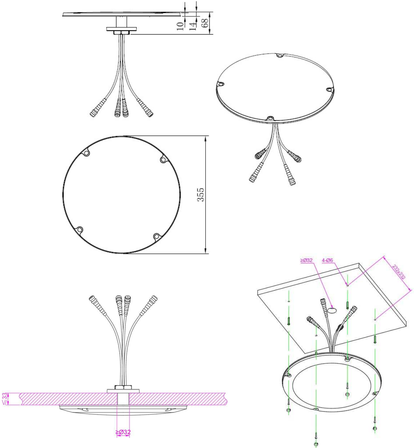
Installation Option 1 Mount on ceiling through locking Nut
